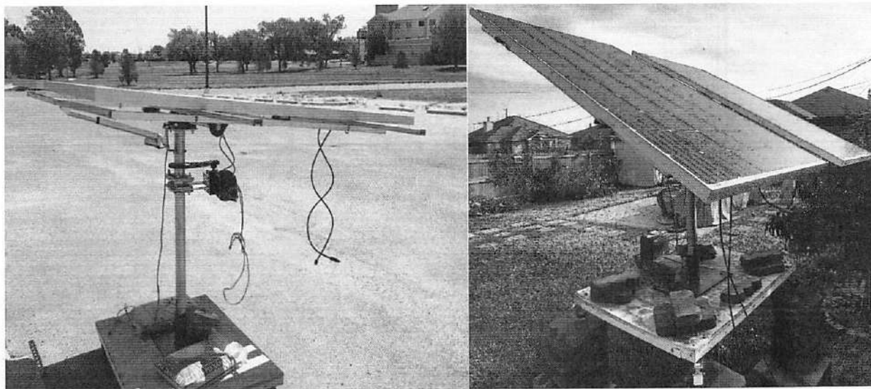
Figure 2. Solar PV prototype with dual axis Sun tracking capability
