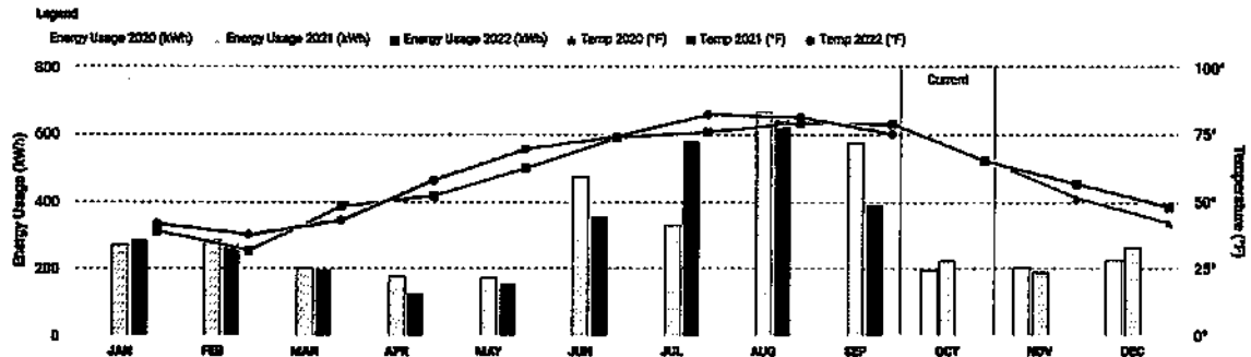
Figure 7. Electricity consumption per month at the house where the research is conducted
