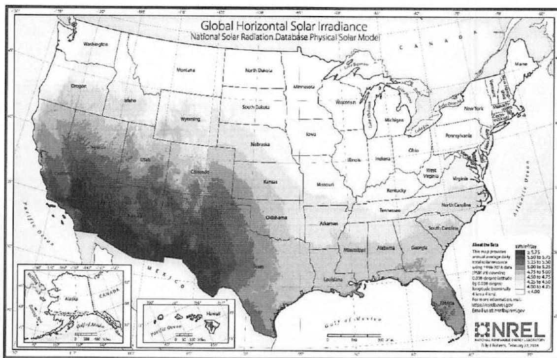
Figure 1. Solar Energy distribution in the United States [2]
