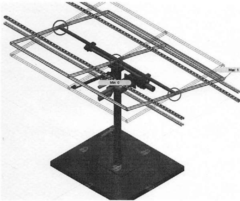
Figure 3. CAD picture of the system during design phase
